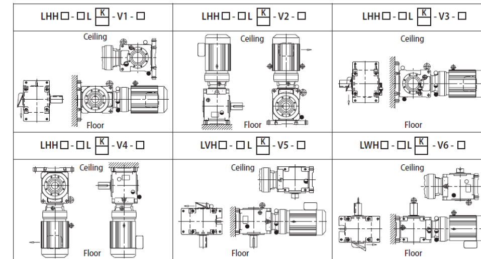
Fig. 2.32 Solid Output Shaft Left (L) - Mounting Foot Side
