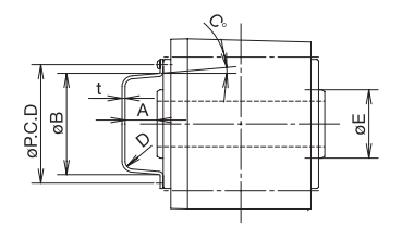
Figure 3.9 Frame Sizes 1200 ~1400
