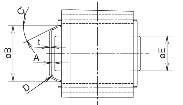
Figure 3.8 Frame Size 1100
