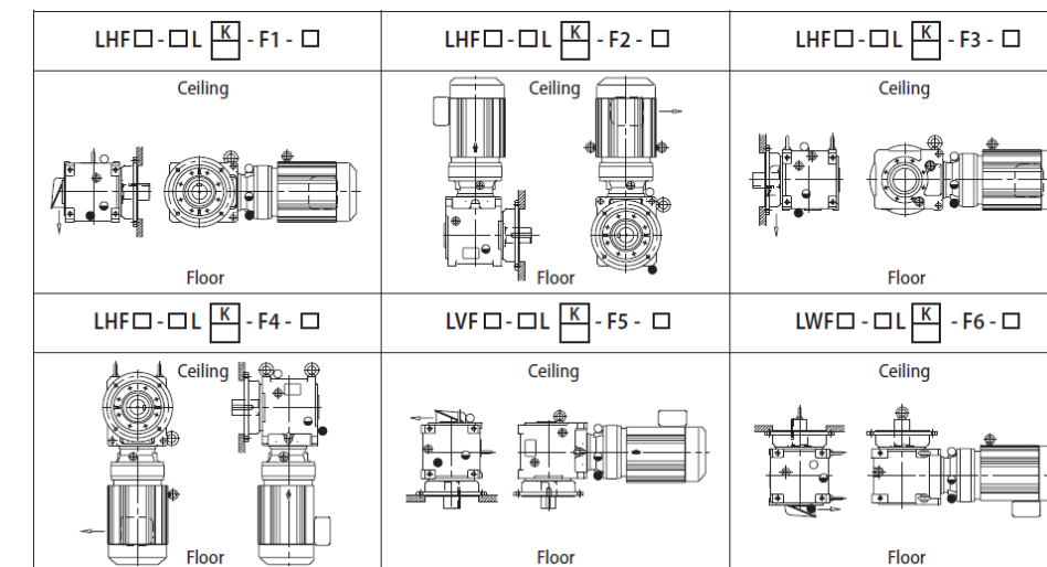
Fig. 2.22 Solid Output Shaft (L) - Output Flange Left
