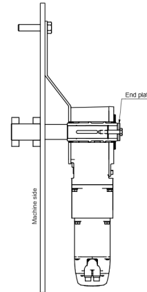
Figure 3.5 Secured by End Plate
